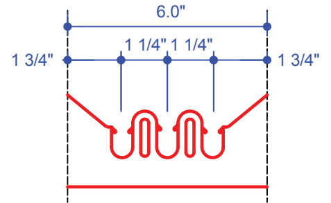
A 1 Typical Block Tie Detail
